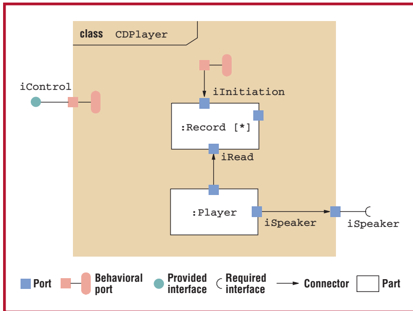
Figure 4. A class's internal structure with behavioral ports.
