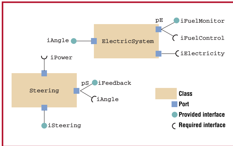
Figure 1. Classes with ports and interfaces.
