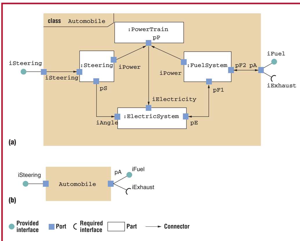
Figure 3. An Automobile class's internal structure (some details omitted): (a) white-box view; (b) black-box view.
