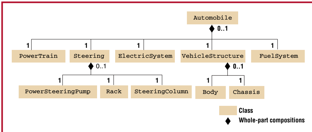
Figure 2. An Automobile class's compositional structure.
